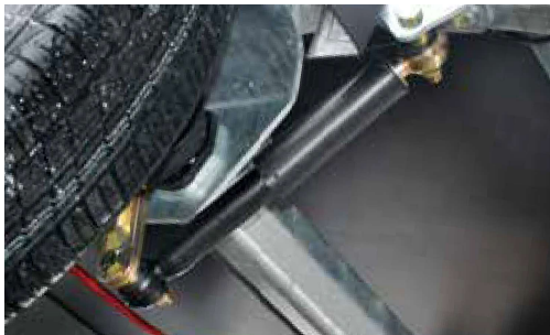
Wheel shock absorbers (mounted), with 100 km/h confirmation; wheel shock absorbers (loose) without 100 km/h confirmation
